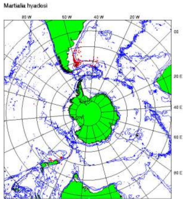
Figure 7: Example of relationship between abundance of Martialia hyadesi (red dots) and bathymetry (data from the Squid Atlas ; www.nerc-bas.ac.uk/public/mlsd/squid-atlas/ ).
