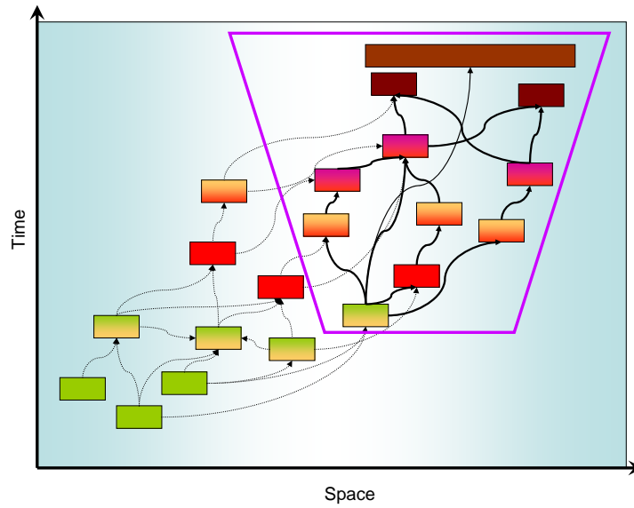
Figure 3: Schematic representation of different taxa and their relationships, within the physical ocean and sea-ice, arranged according to the spatial and temporal scales within which individuals of the different taxa typically function. The trapezoid shows a typical subset of a minimal realistic model that might be considered by CCAMLR and the IWC with krill at the bottom of the food web operating at smaller scales than larger predators. In this case, some species of whales cover broad spatial scales and are shown at the top of this food web.
