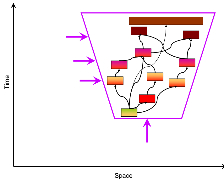
Figure 4: For simplicity, the food web and physical environment outside the trapezoid is then collapsed into a series of forcing functions indicated by the arrows.
